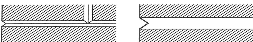
Keyed pointing
